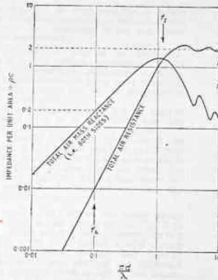
Fig. 3. Mass and radiation resistance curves for a circular diaphragm in a large baffle. The power radiated at any frequency f_A well below f_0 is half that radiated at frequencies f_B well above f_0 (see text).
