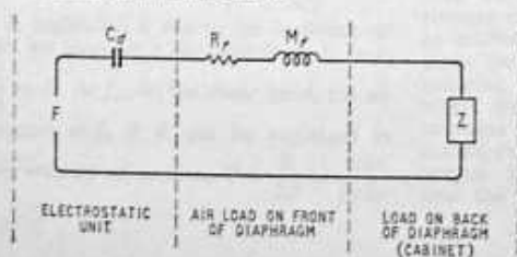
Fig. 1. Elementary equivalent circuit of mechanical and acoustical parameters of an electrostatic loudspeaker.
